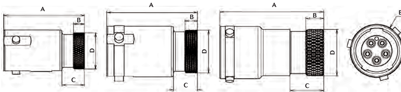
Shell size 3
