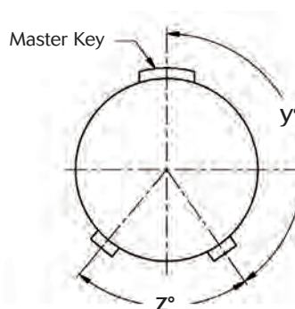
Shell size 5 & 7
